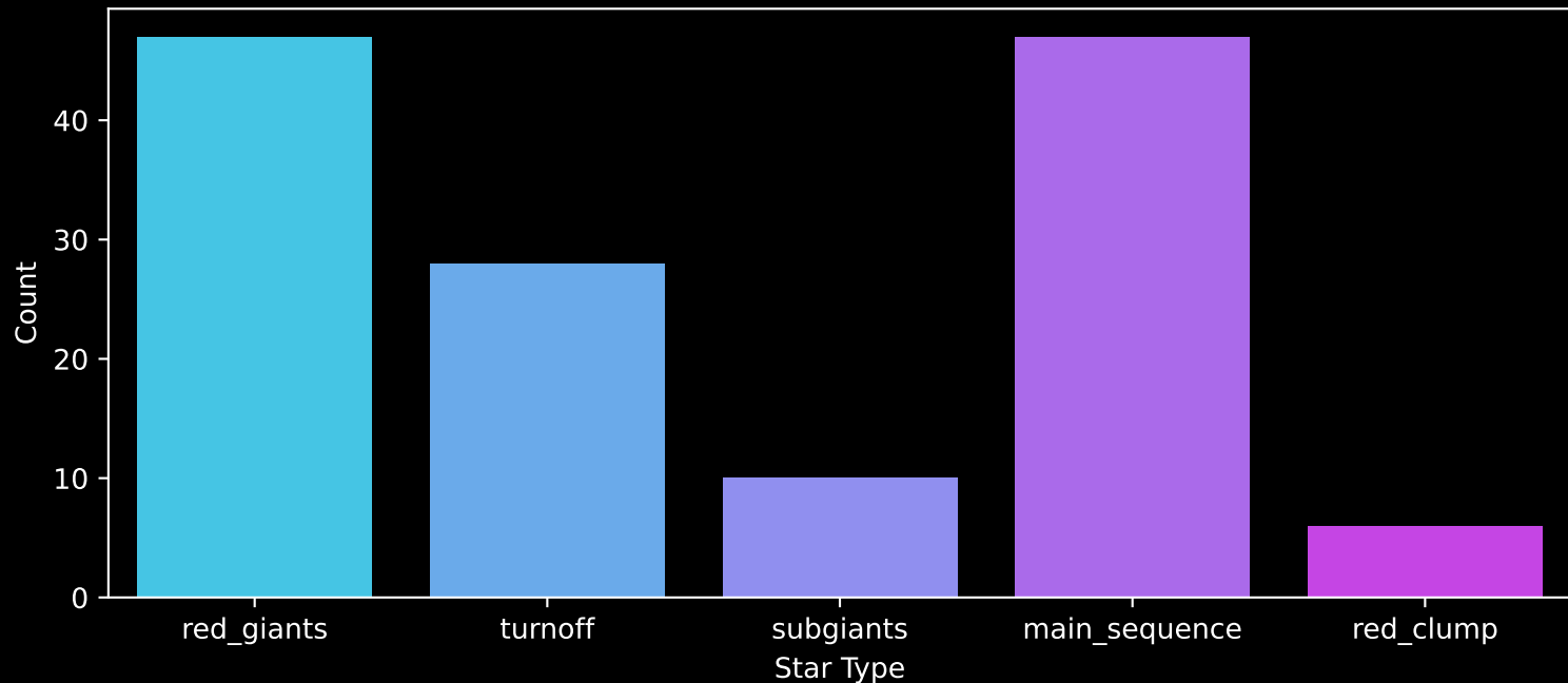
APOGEE DR17 Field: [278-29-O_TESS] Count plot of Star Type
