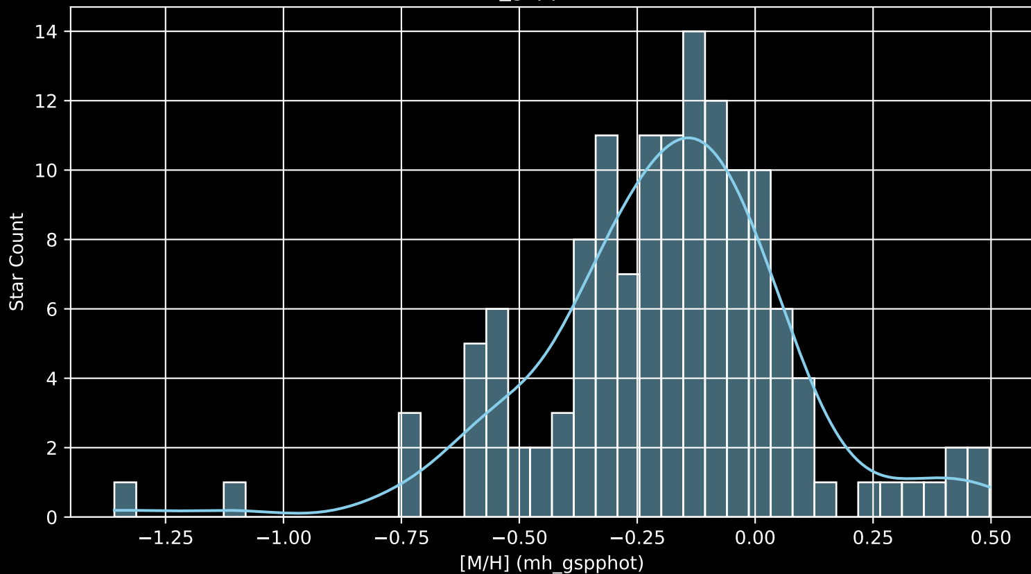
APOGEE DR17 Field: [278-29-O_TESS [M/H] (mh_gspphot) (n= 136)
