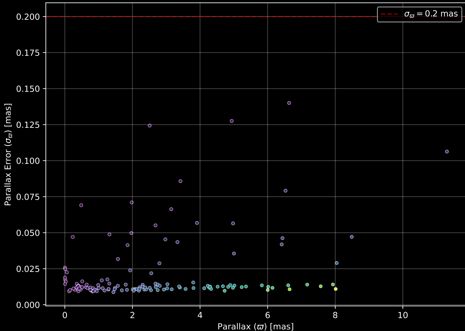
APOGEE DR17 Field: [278-29-O_TESS] Parallax Quality (n= 138)
