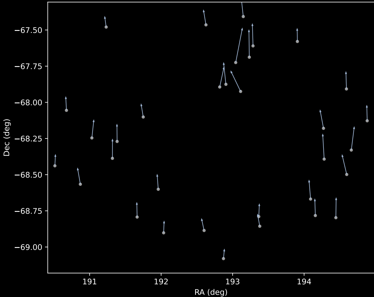
APOGEE DR17 Cluster 1 Proper Motion Vectors (n=33)
