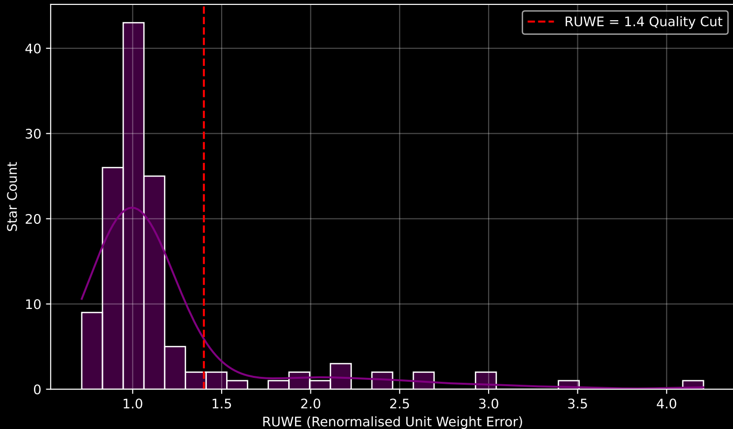
GAPOGEE DR17 Field [278-29-O_TESS] RUWE Distribution (n= 128)
