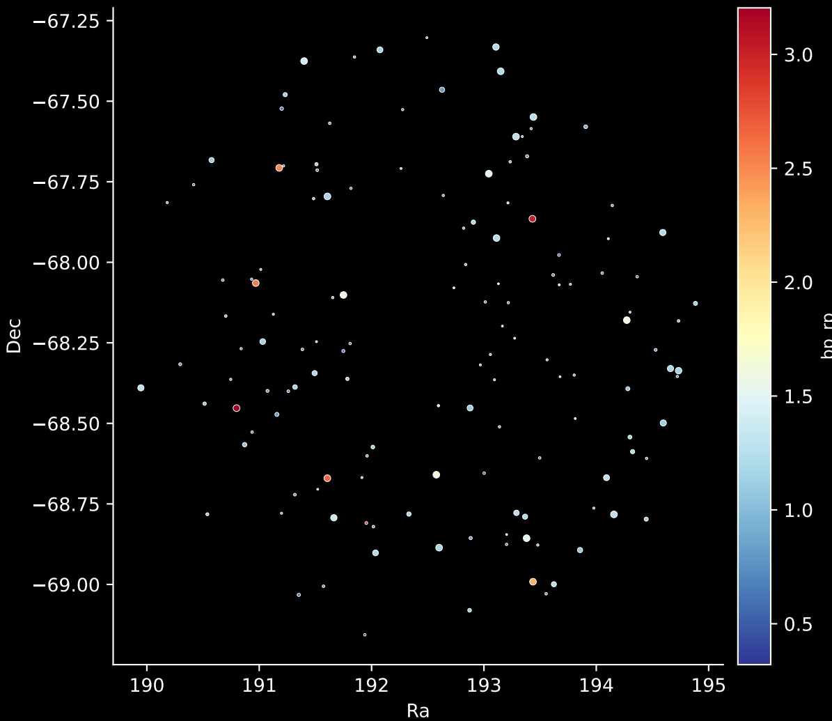
APOGEE DR17 Field: [278-29-O_TESS] Stars: 138
