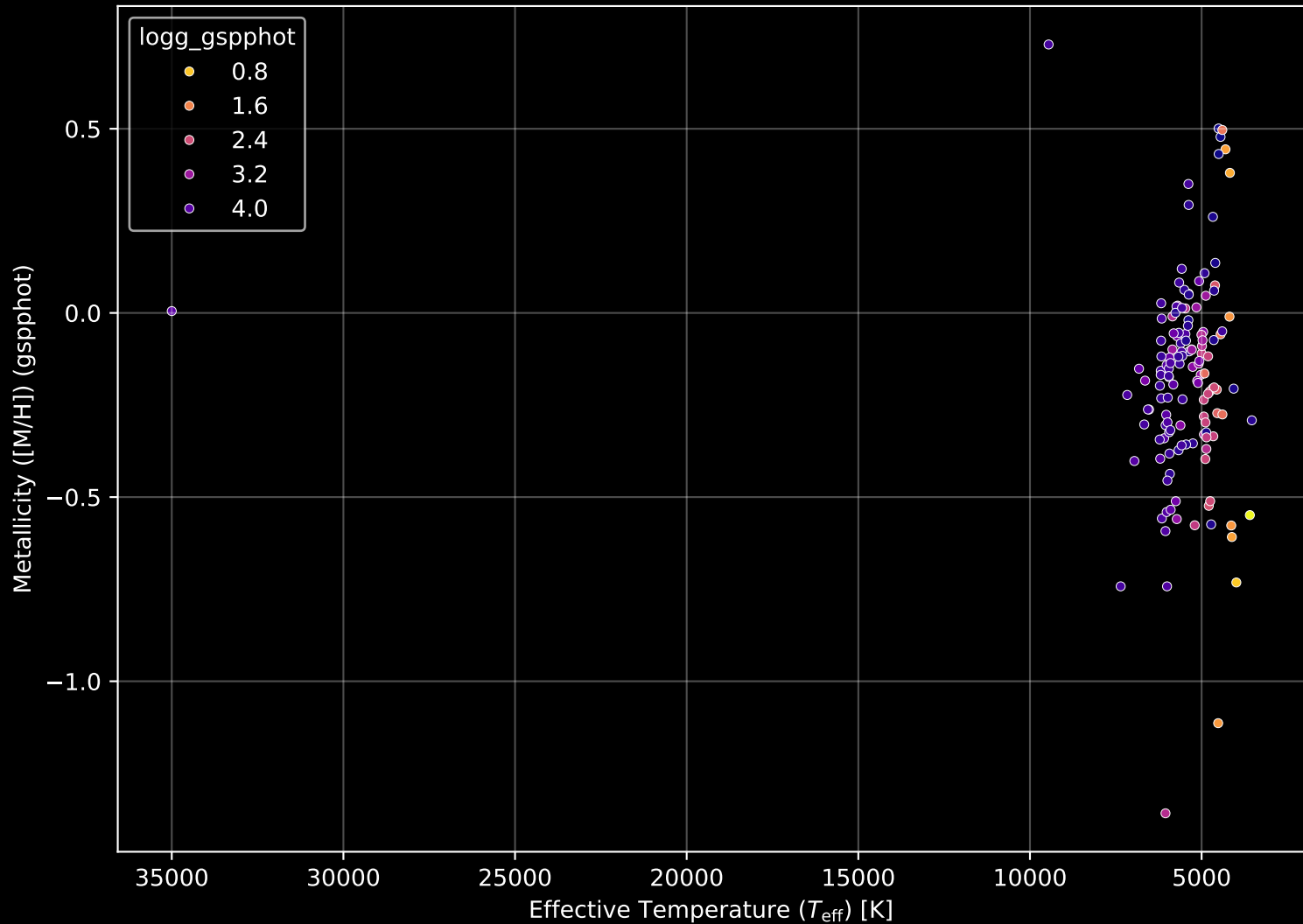
APOGEE DR17 Field: [278-29-O_TESS] Stellar Population Parameters (n= 138)
