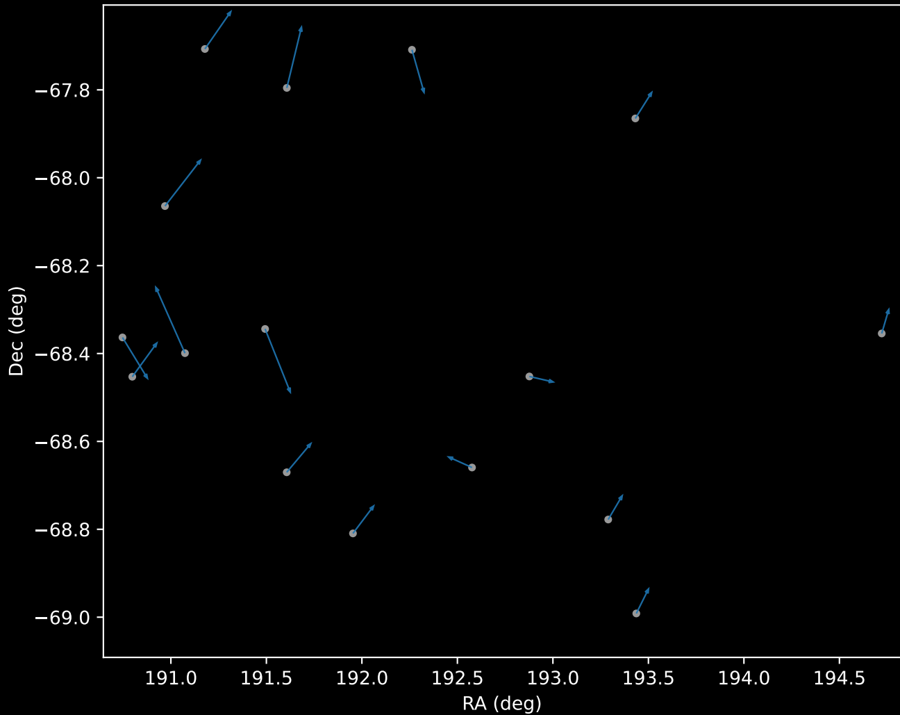
APOGEE DR17 Cluster 0 Proper Motion Vectors (n=16)
