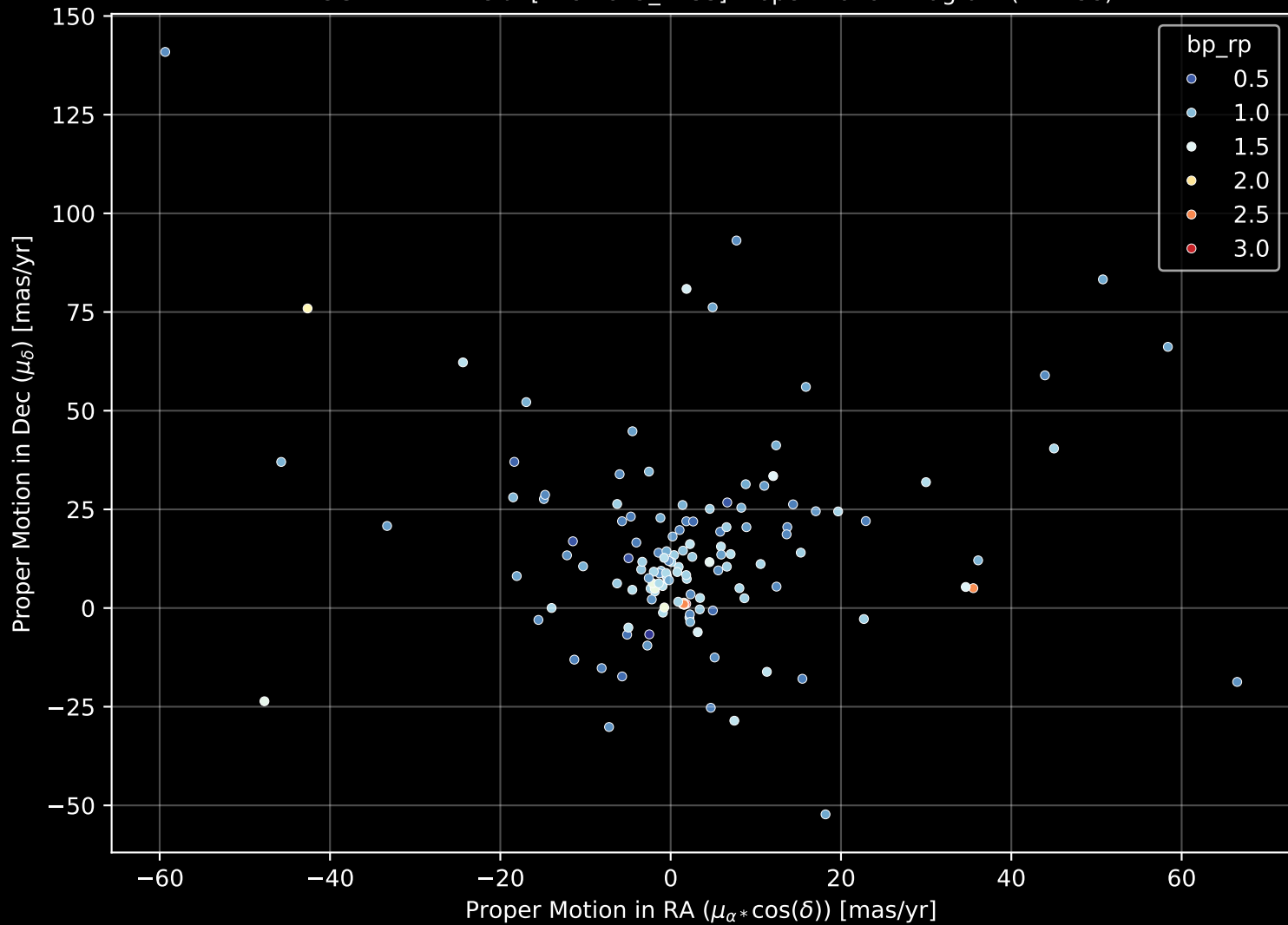
APOGEE DR17 Field: [278-29-O_TESS] Proper Motion Diagram (n= 138)
